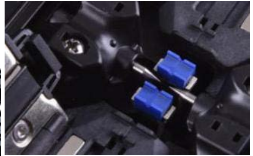
3-in-1 Universal Holder 15 seconds Speedy Heating Applicable Cleaved Length up to 5mm
