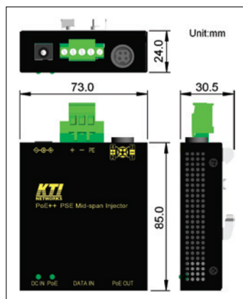
DIN-Rail Dimension
