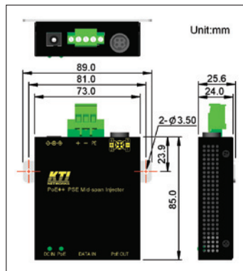
Panel Dimension
